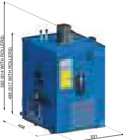
TORNADO EVOLUTION 15/L
