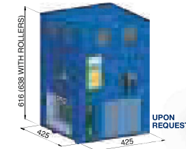
TORNADO EVOLUTION 25/L CARENATO/CASING
