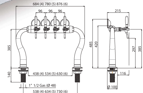
MAYA A PONTE 4 VIE/BRIDGE 4 WAYS C642-3
