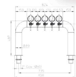
AZUR A PONTE / BRIDGE C767-4
