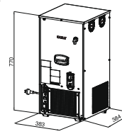
GEO 30/L VERTICALE CARENATO VERTICAL CASING
