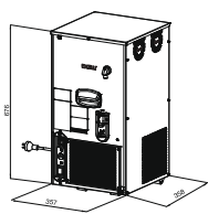
GEO 20/L VERTICALE CARENATO VERTICAL CASING
