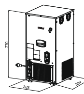
GEO 30/L VERTICALE CARENATO VERTICAL CASING
