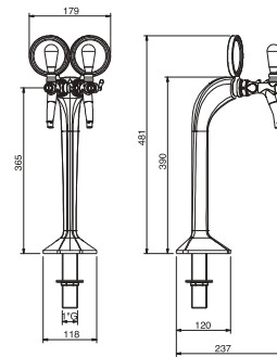
COBRA® CLASSIC 2 C000103-004
